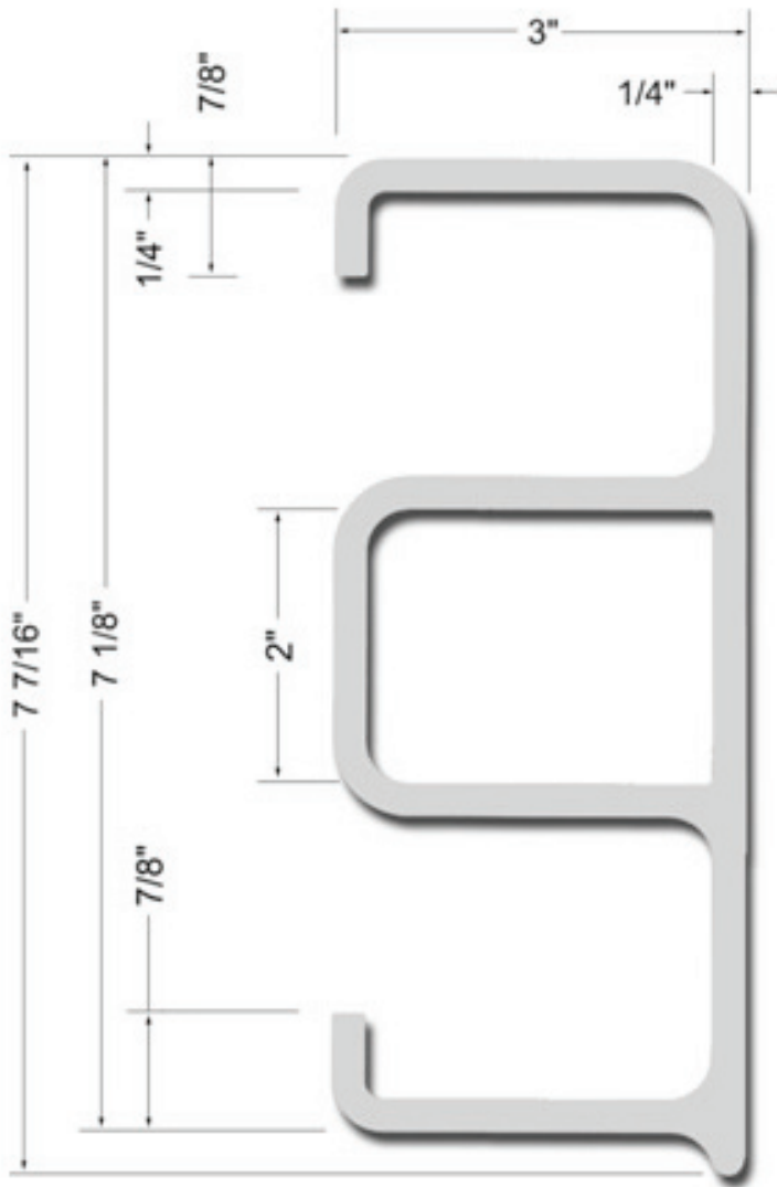
HMAX Extreme Duty Flight - 8"
